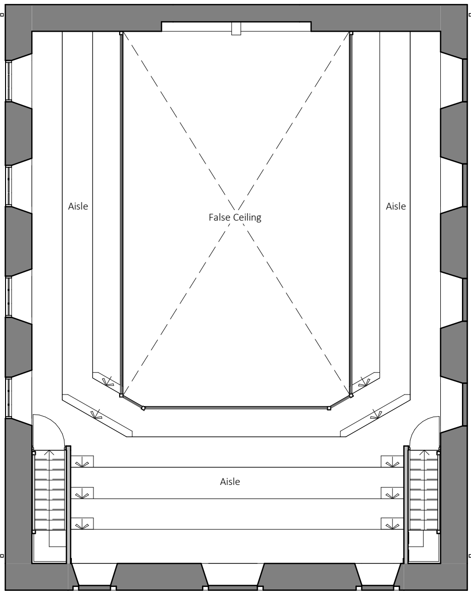
First Floor
