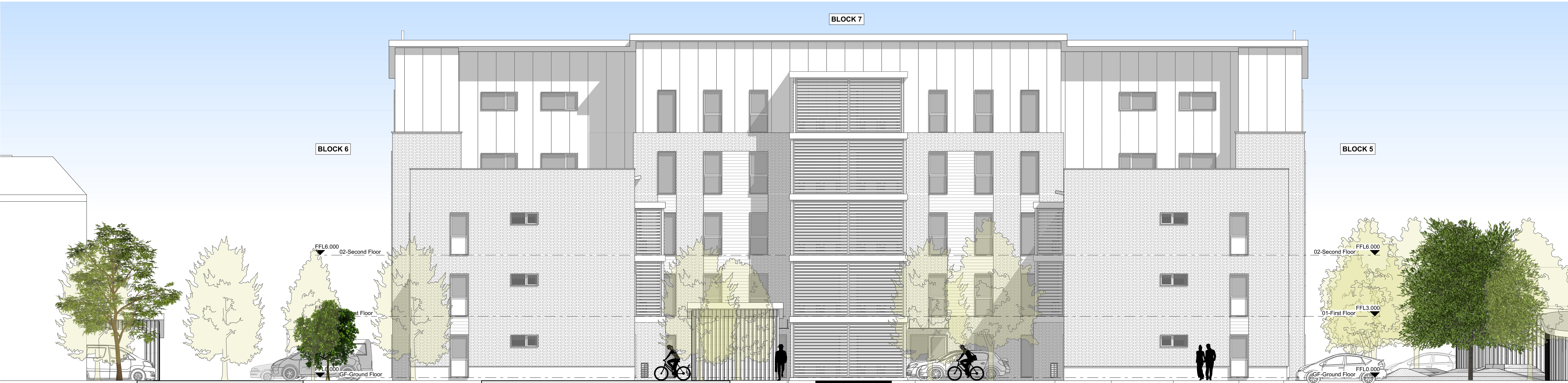
E-03 Moorland Road Elevation
