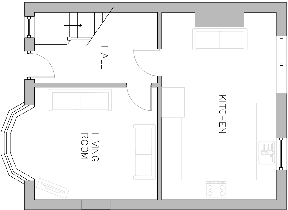
EXISTING GROUND FLOOR PLAN SCALE - 1:50 @ A3
