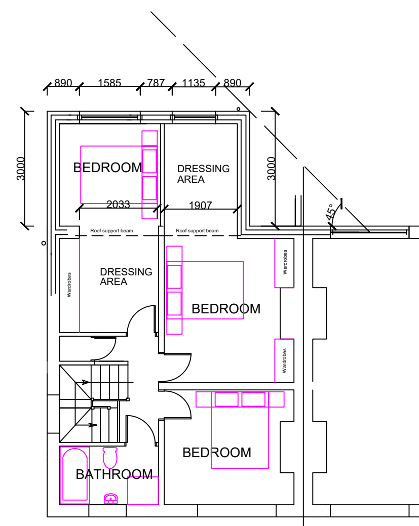
PROPOSED FF PLAN
