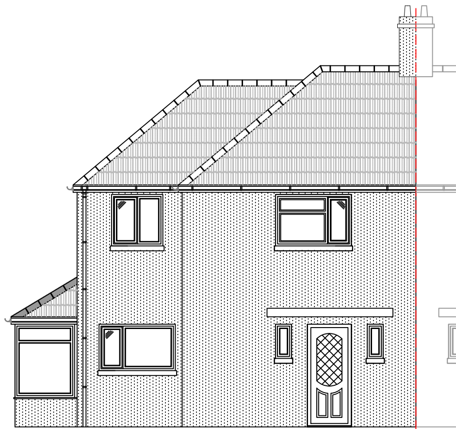
EXISTING FRONT ELEVATION 1:75
