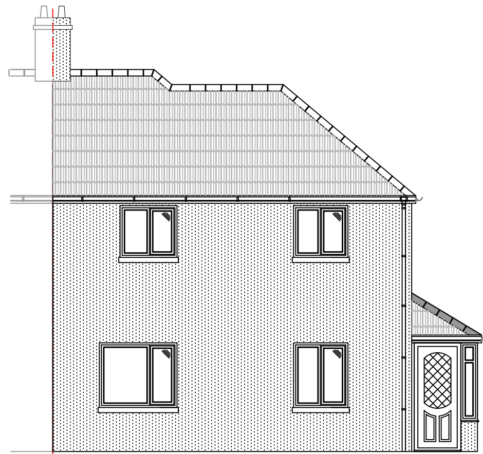
EXISTING REAR ELEVATION 1:75
