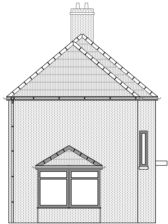
EXISTING LEFT ELEVATION 1:75
