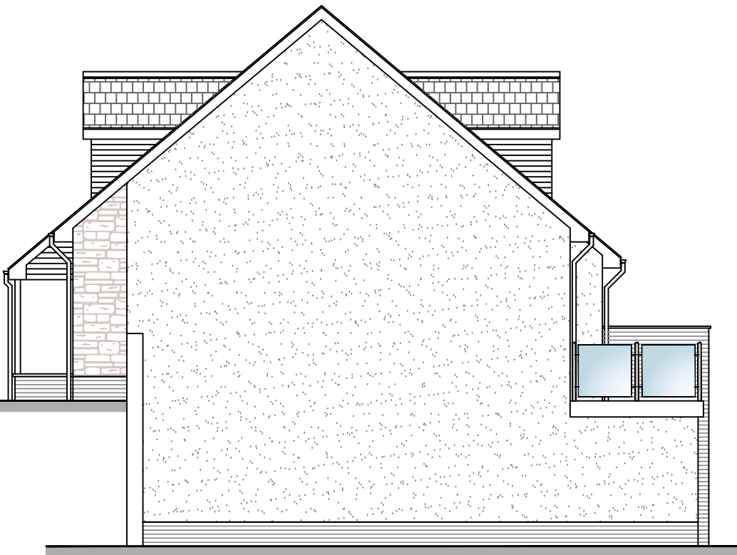
Side Elevation
