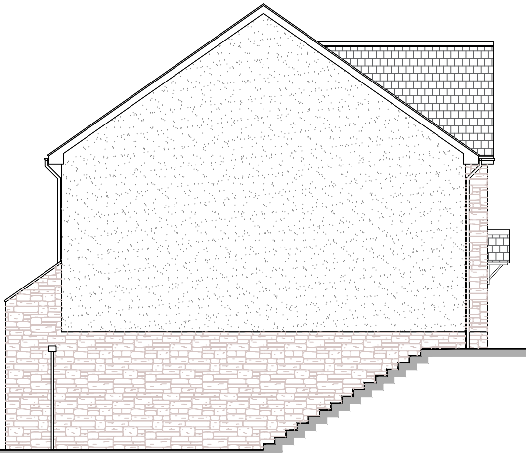
Side Elevation
