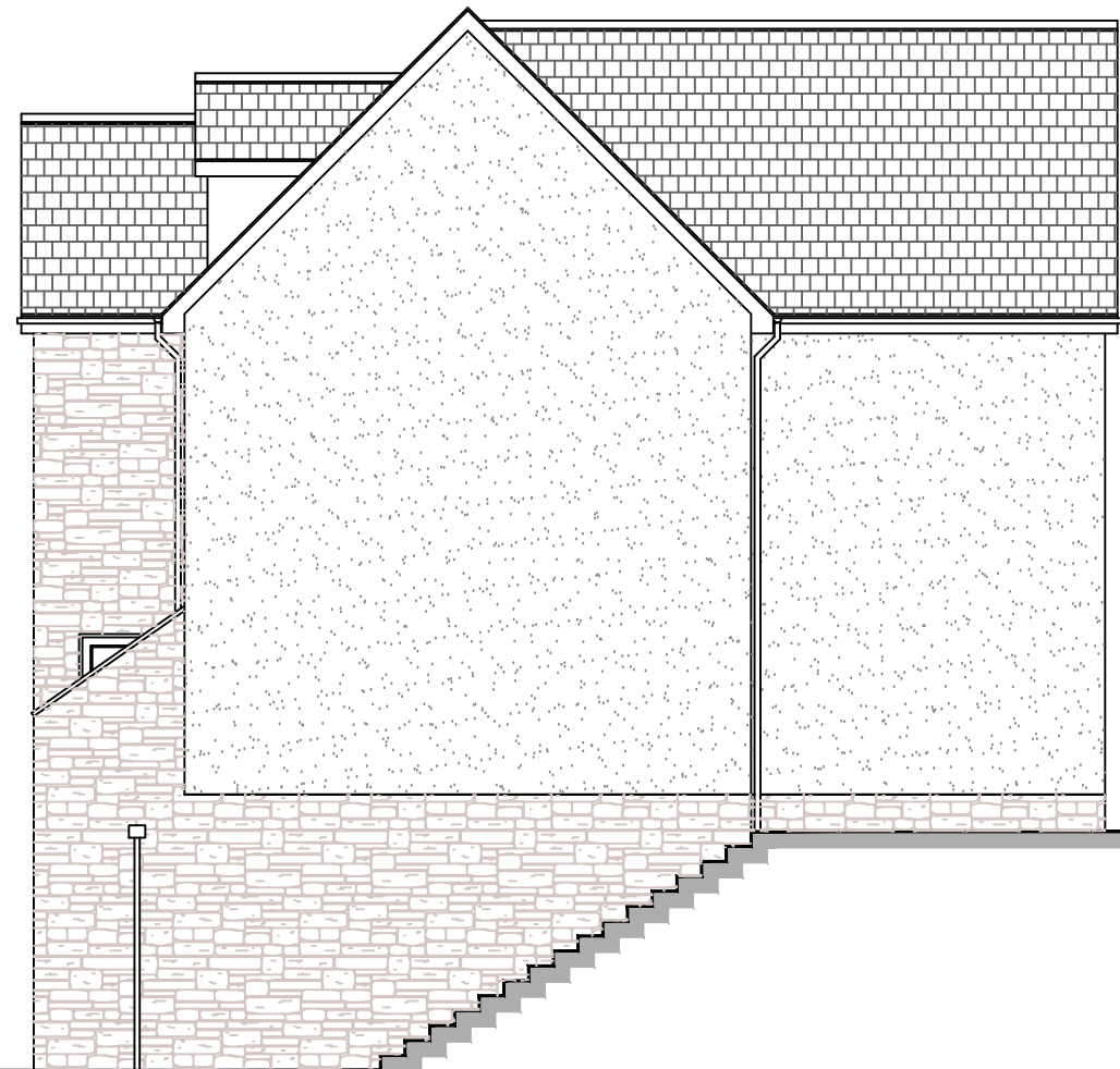
Side Elevation
