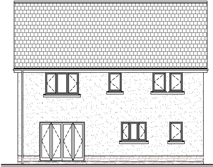
Rear Elevation
