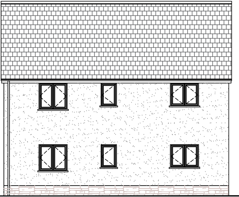
Rear Elevation
