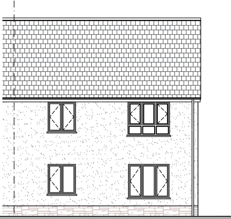
Rear Elevation
