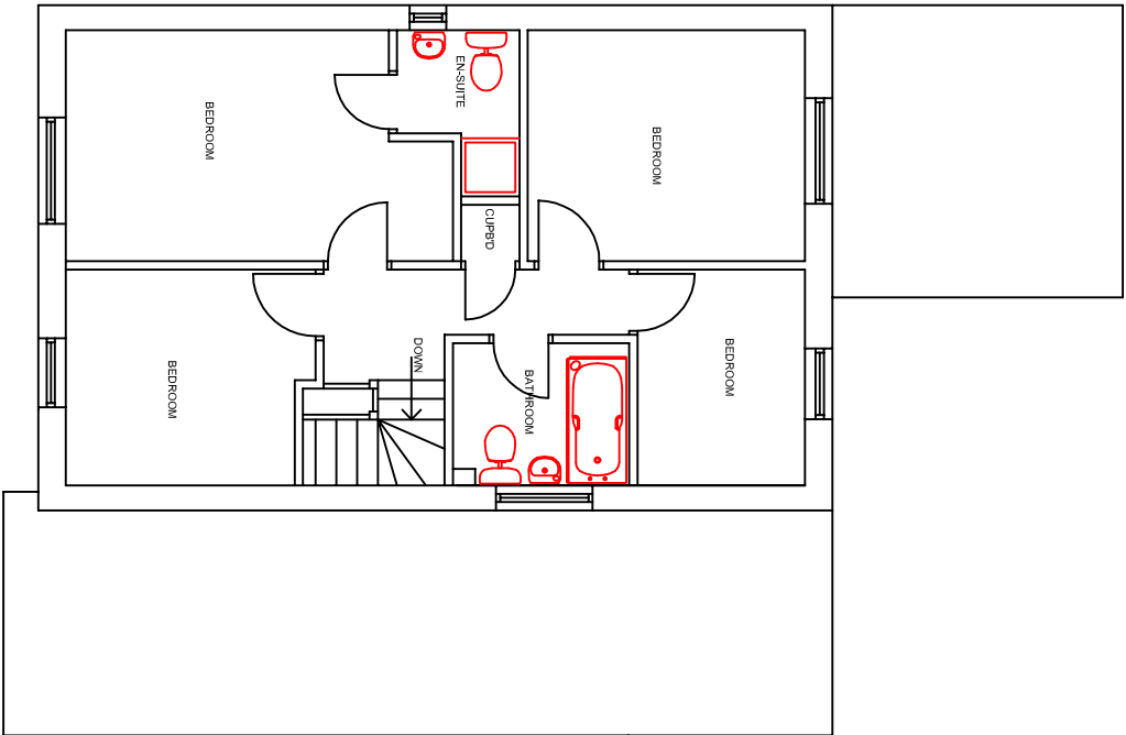
EXISTING FIRST FLOOR LAYOUT SCALE 1:100
