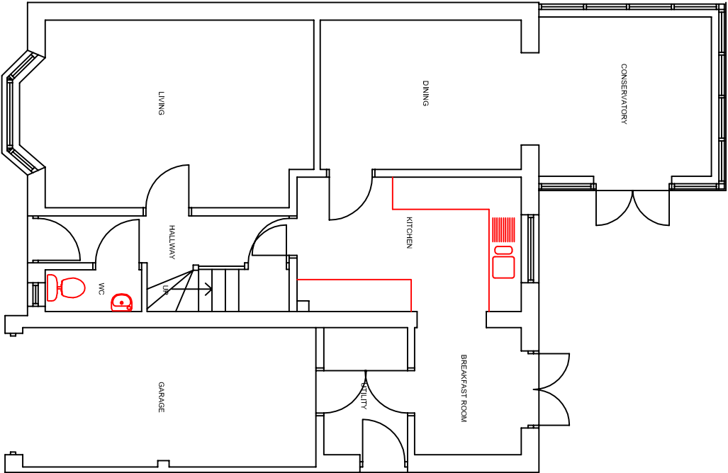
EXISTING GROUND FLOOR LAYOUT SCALE 1:100
