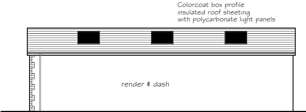
RH Side Elevation
