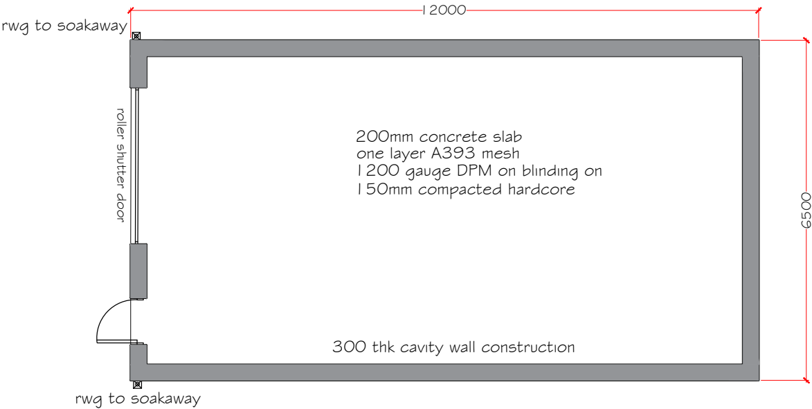
Floor Plan
