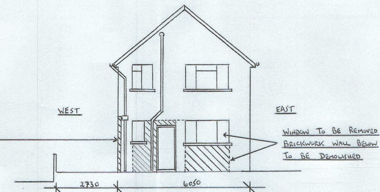
EXISTING REAR (SOUTH) ELEVATION 1:100
