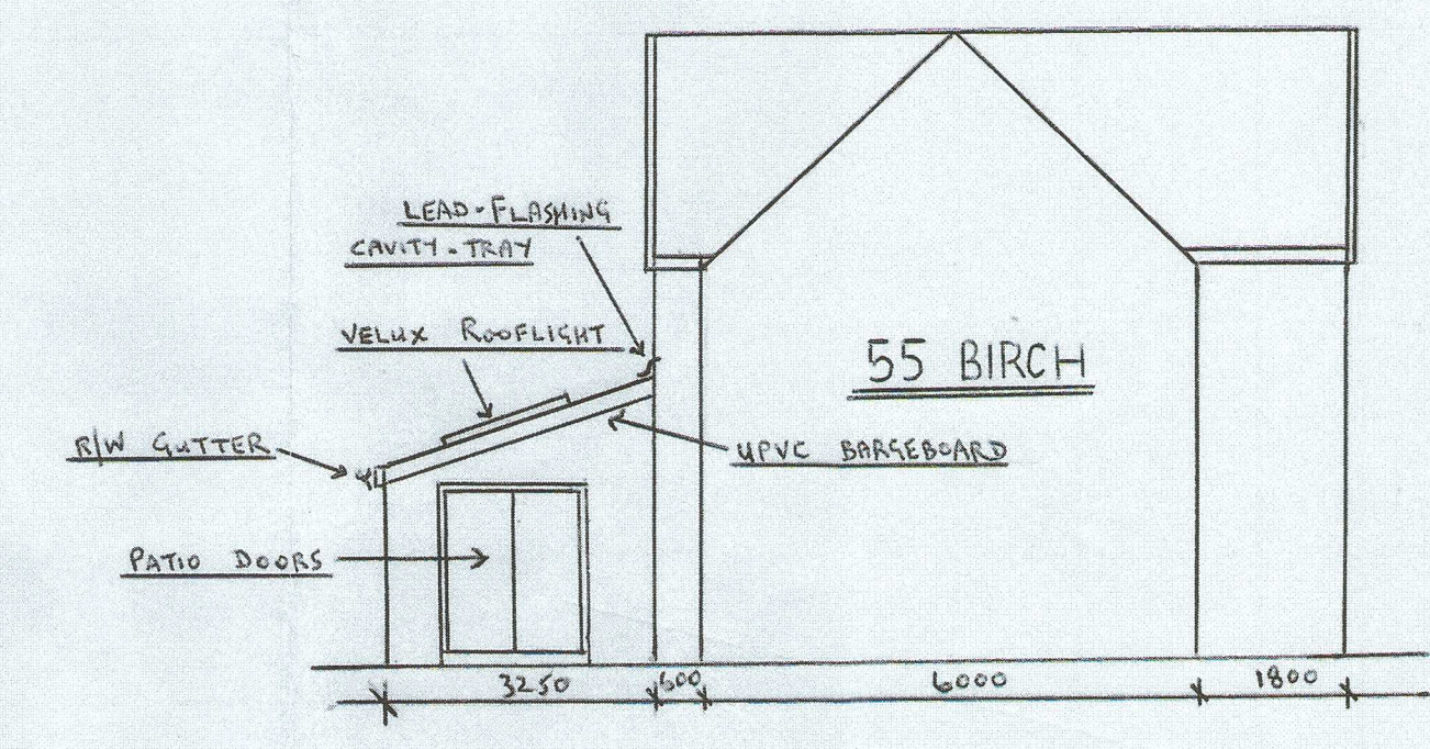
PROPOSED SIDE (EAST) ELEVATION 1:100
