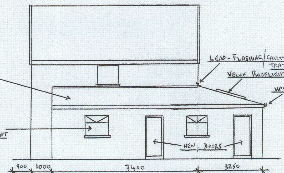
PROPOSED SIDE (WEST) ELEVATION 1:100
