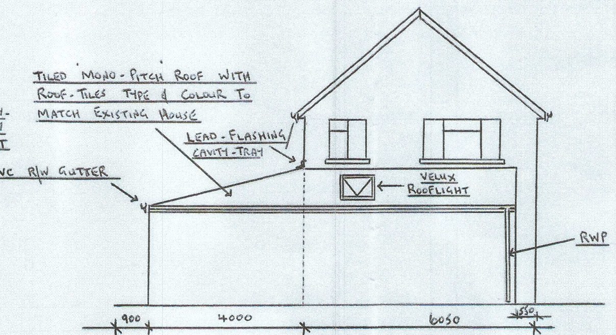
PROPOSED REAR (SOUTH) ELEVATION 1:100
