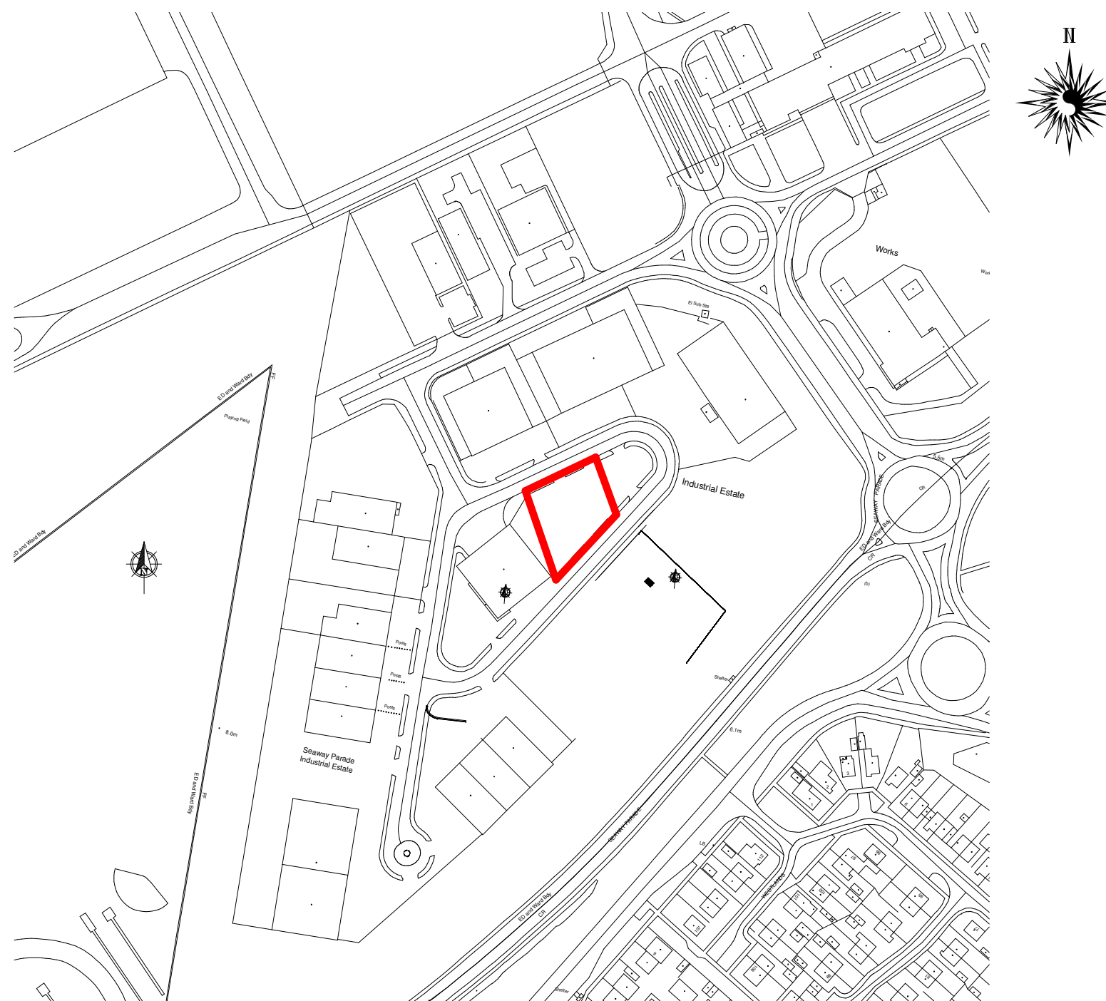
LOCATION PLAN. . 1 : 2500
