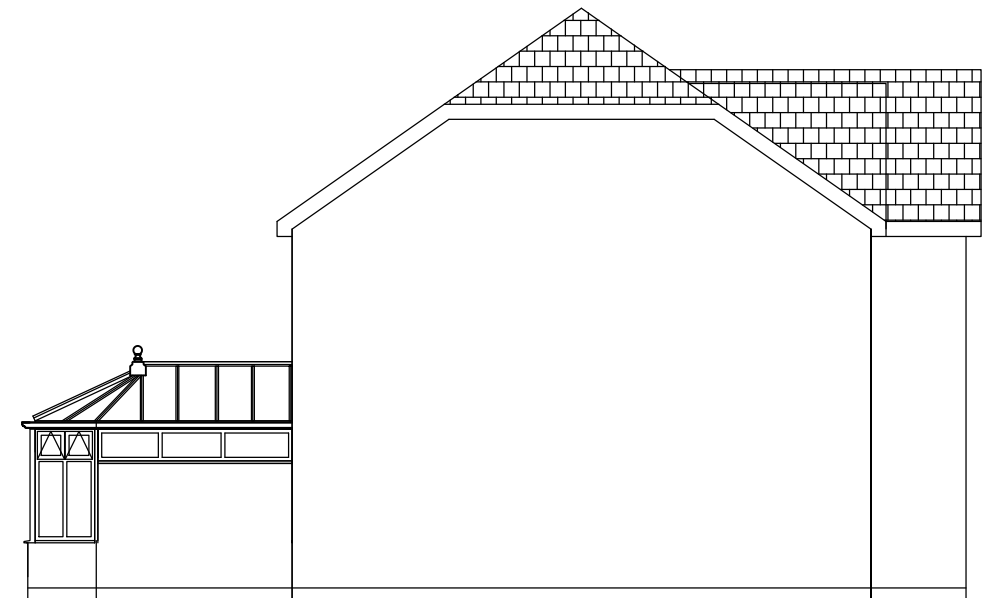
Existing Right elevation
