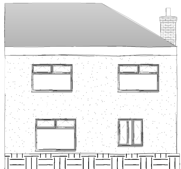
South 1 : 100
