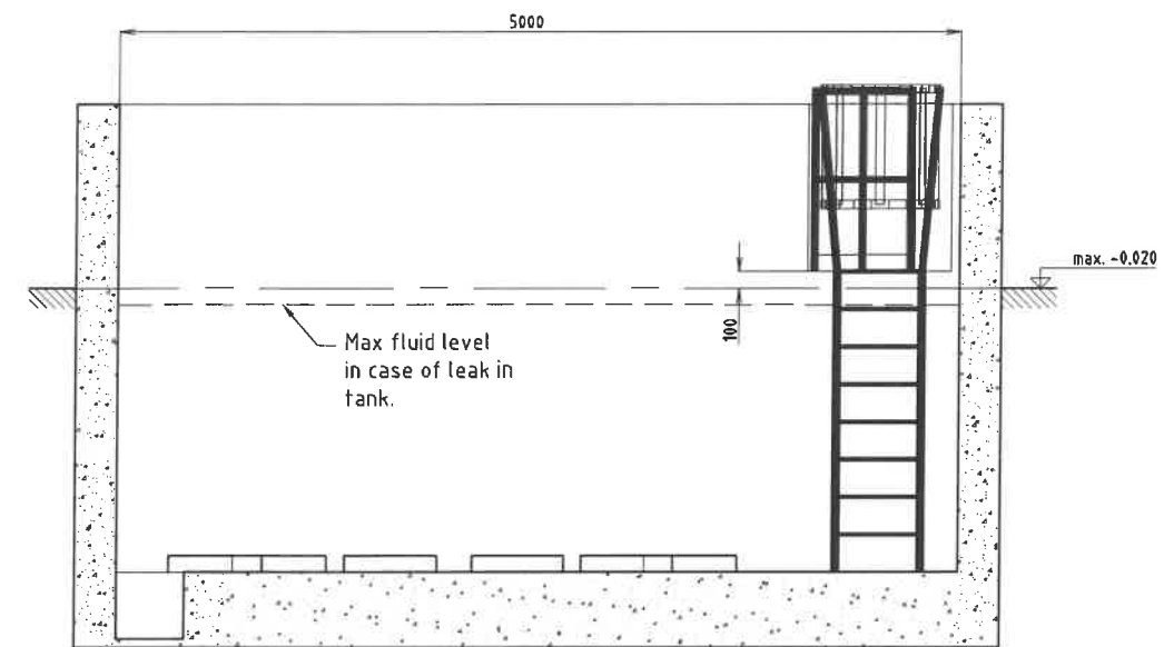
View B-B
