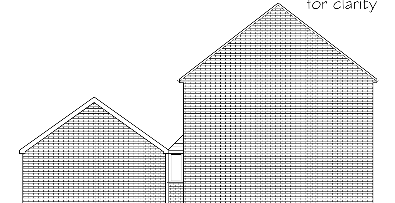
Existing RH Side Elevation
