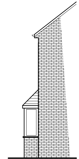
Existing RH Side Elev. garage not shown for clarity
