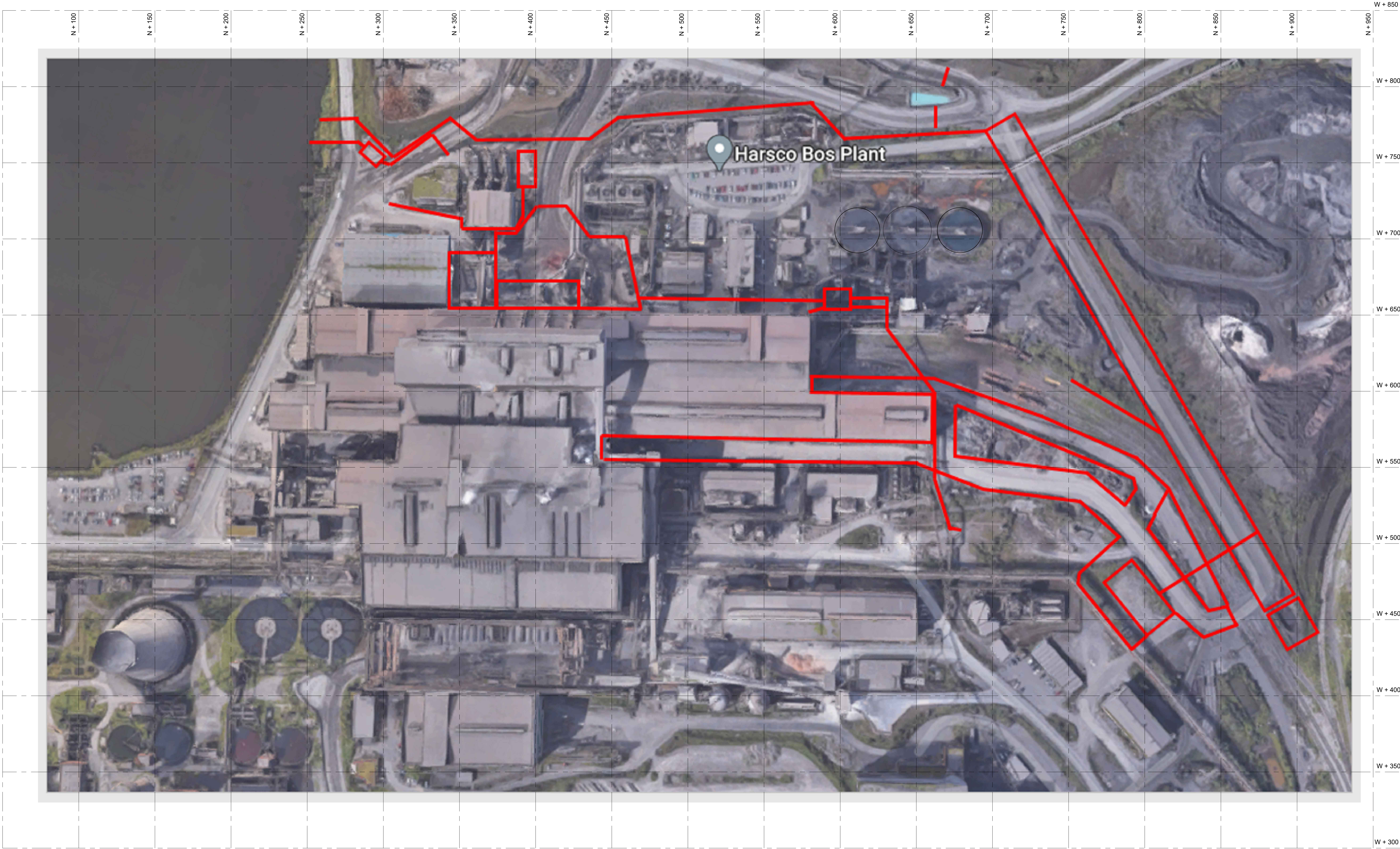
BOS PLANT AREA LAYOUT SCALE 1:1000
