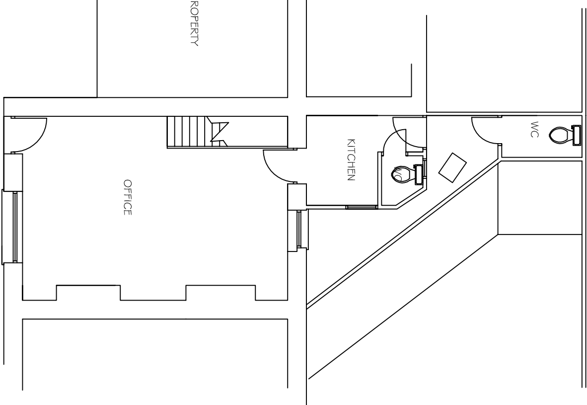
PR. GROUND FLOOR PLAN
