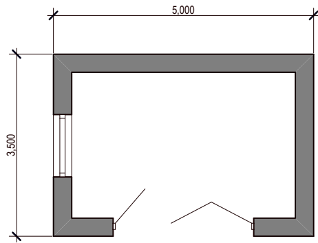
Floor Plan
