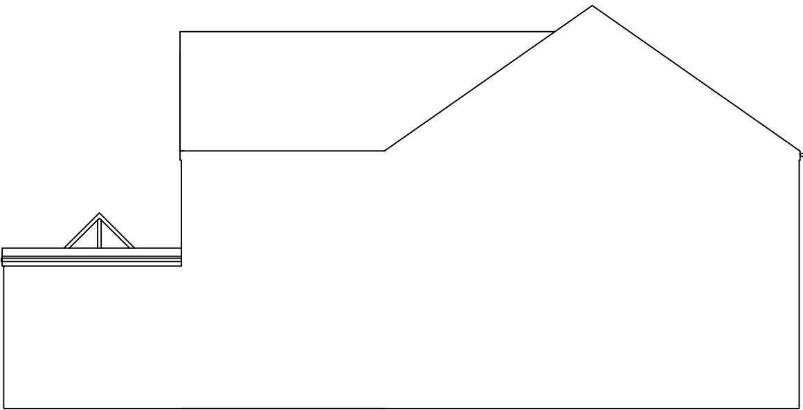
PROPOSED SECTIONAL END ELEVATION
