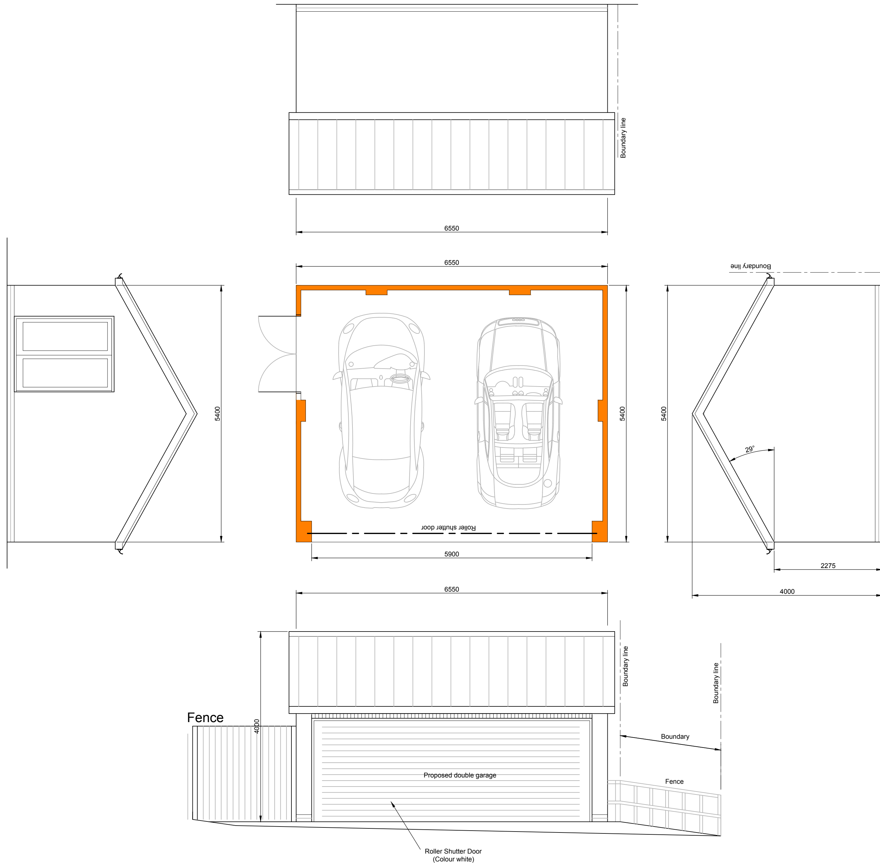
Proposed Double Garage (Scale 1:50)
