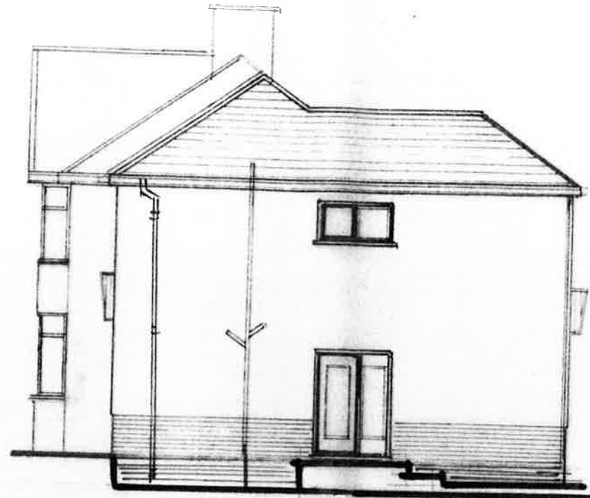
EXISTING SIDE
