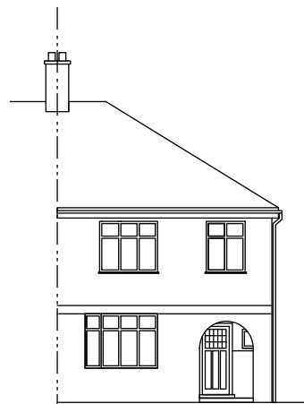
FRONT ELEVATION @1.200
