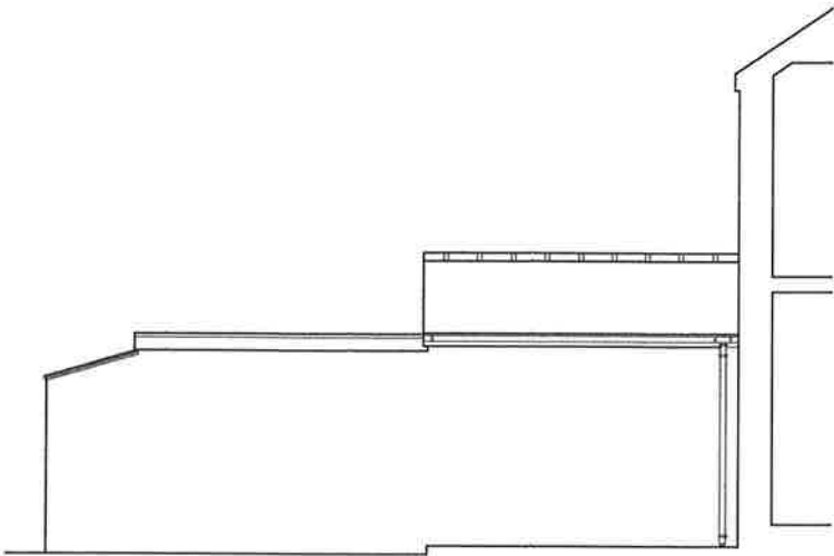
Existing Side Elevation ( from No. 18 )
