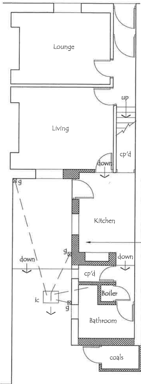
Existing Ground Floor Layout
