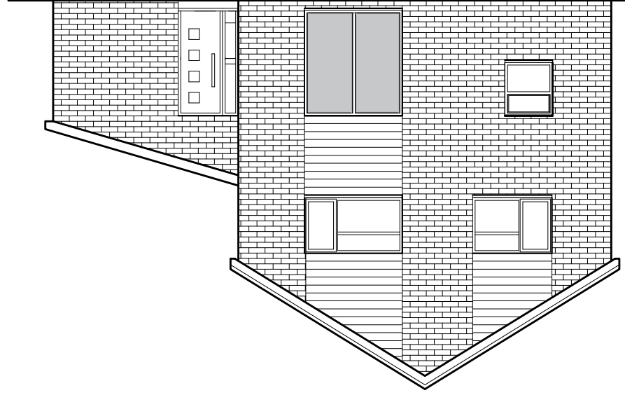
Proposed Elevation RHS
