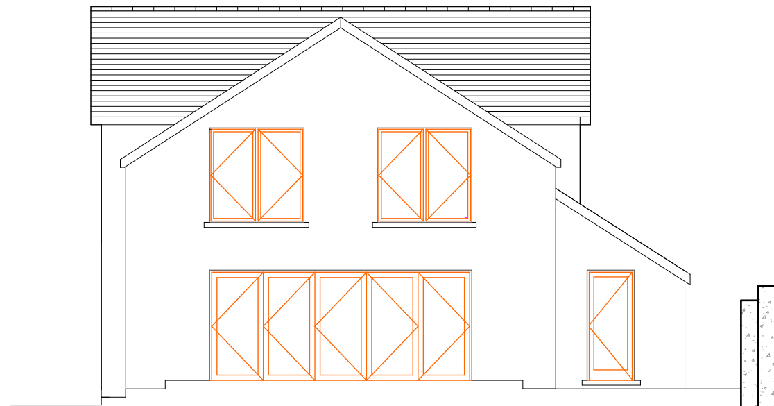
BACK ELEVATION
