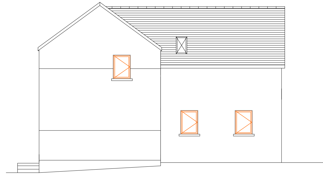
SIDE ELEVATION
