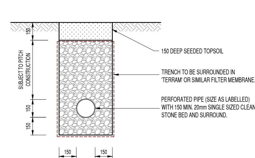
PRIMARY LAND DRAIN TO 2G HOCKEY PITCH SCALE 1:20
