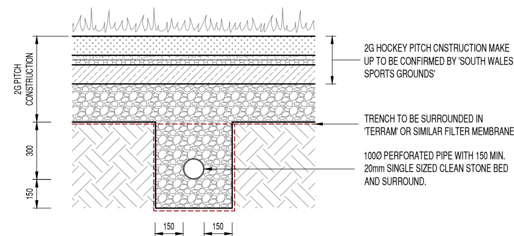
SECONDARY LAND DRAIN BELOW 2G HOCKEY PITCH SCALE 1:20
