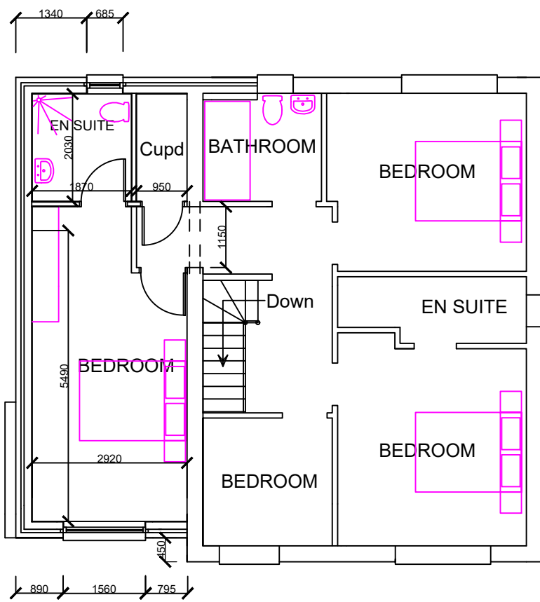
PROPOSED F.F. PLAN
