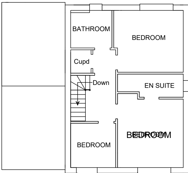
EXISTING F.F. PLAN
