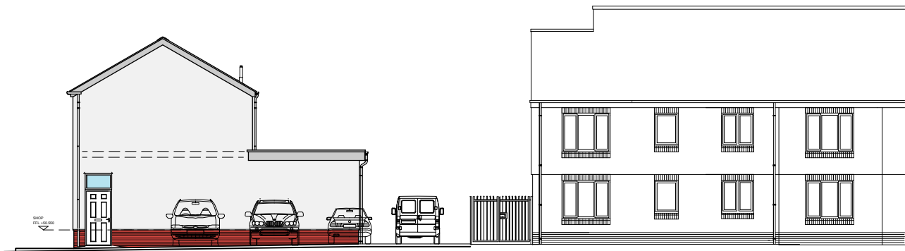
PROPOSED STREET ELEVATION TO ANGEL STREET
