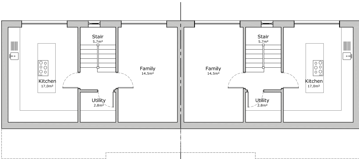
Lower Ground - 41.5m²
