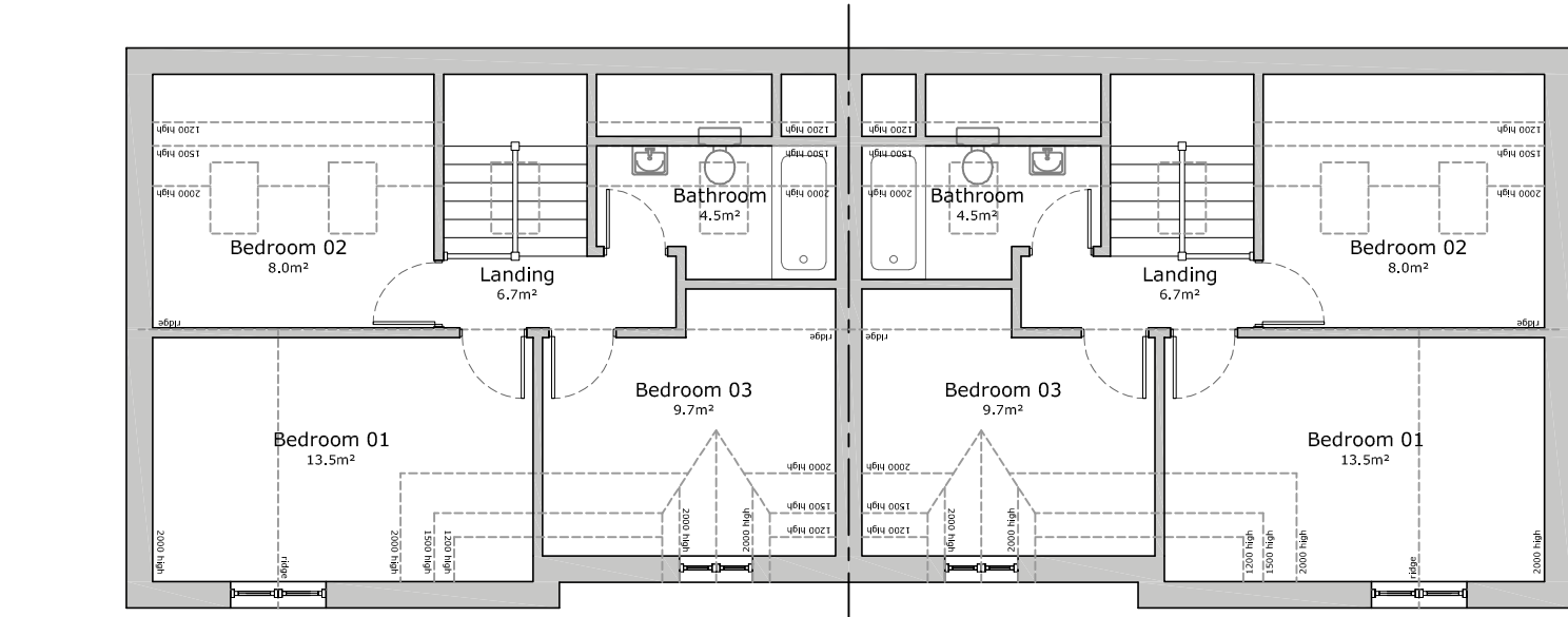
First Floor - 43.0m²
