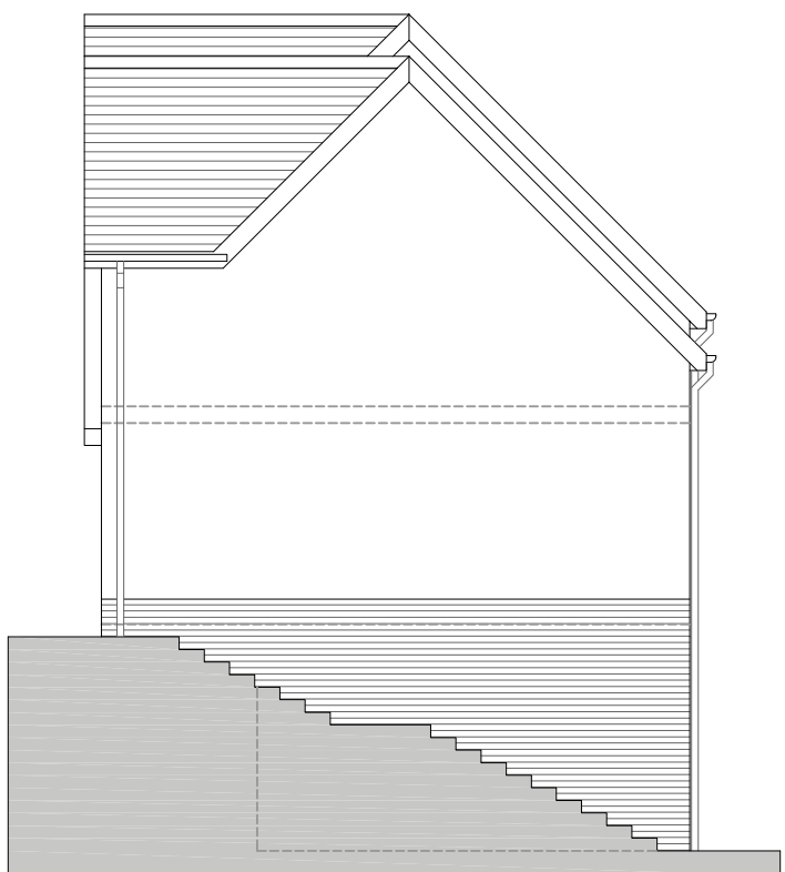
Side Elevation
