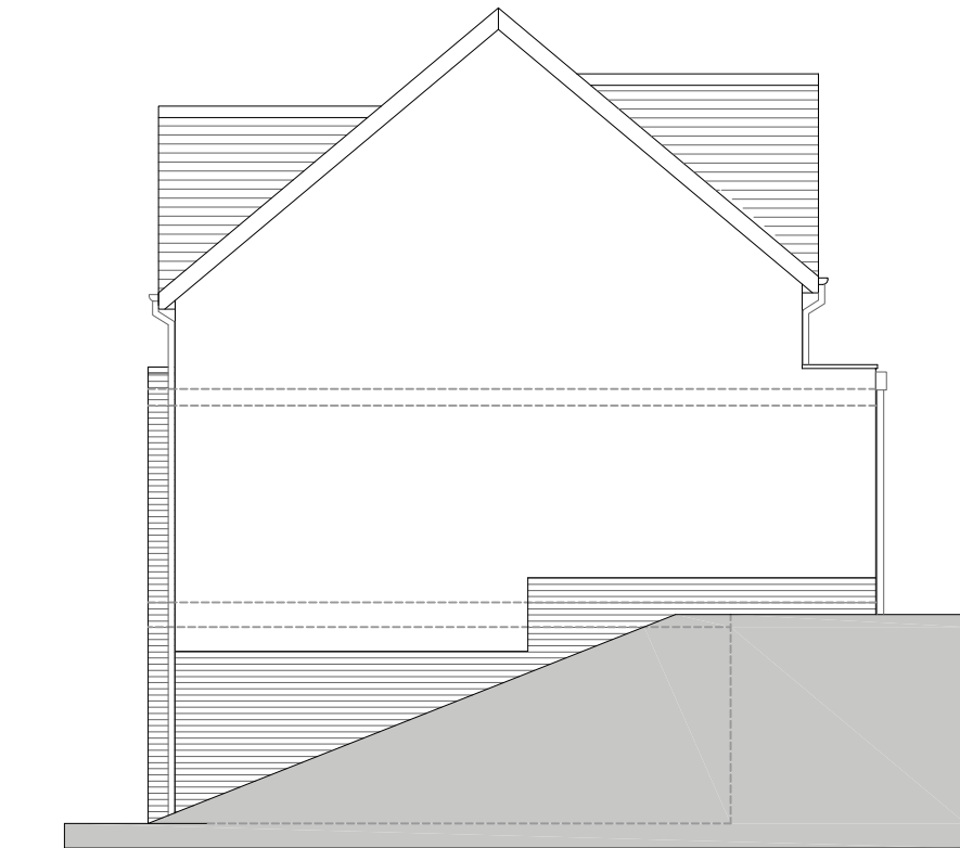
Side Elevation
