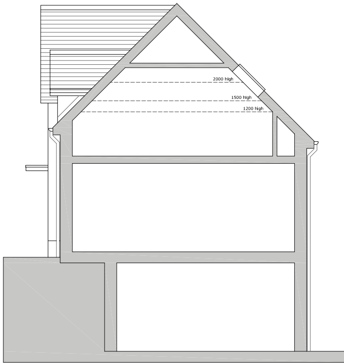
Section
