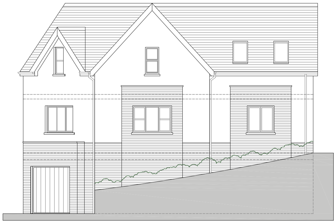
Front Elevation (to Pen Yr Alltwn)
