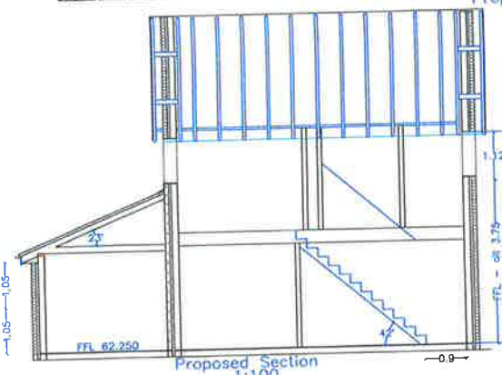
Proposed Section 1:100
