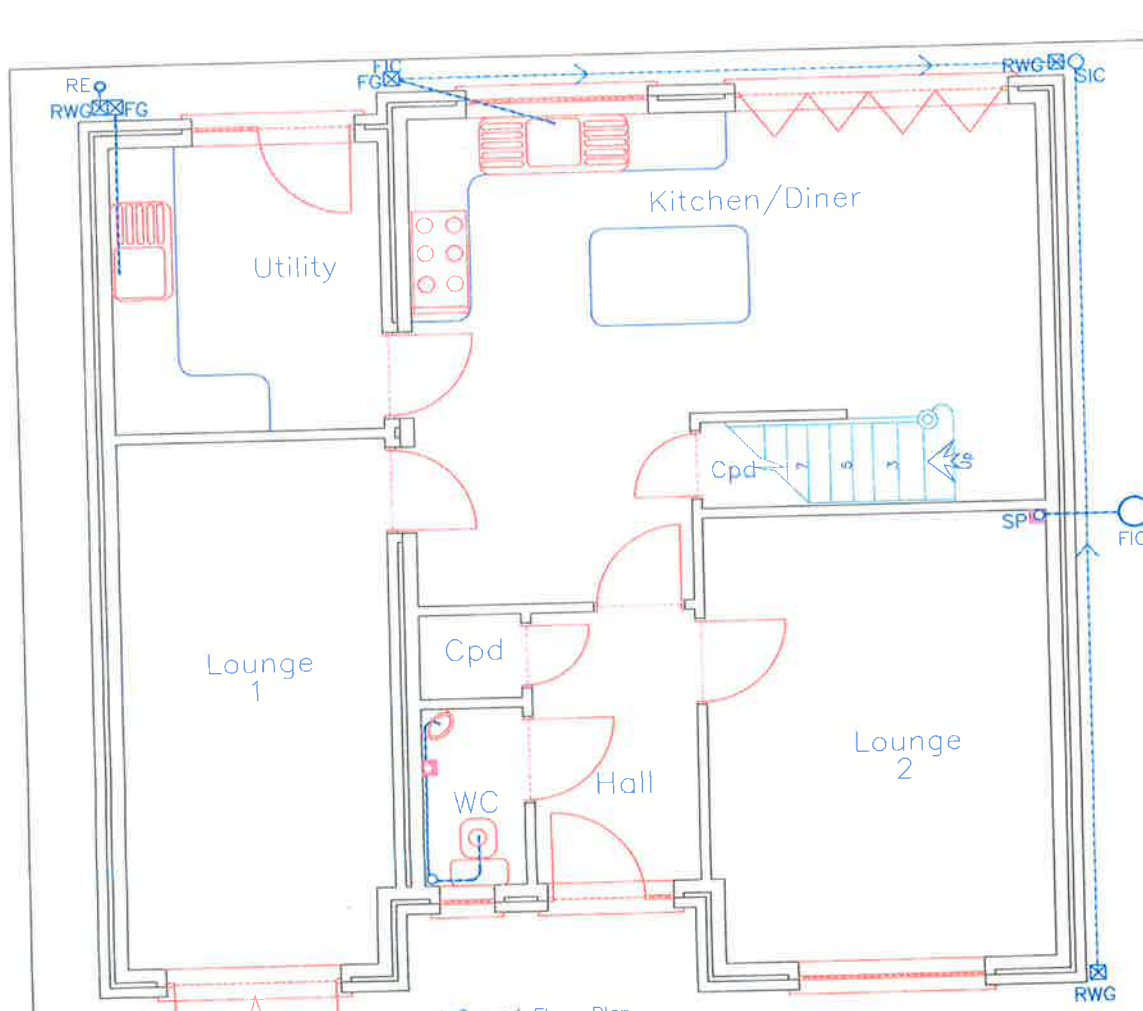
Proposed Ground Floor Plan 1:50
