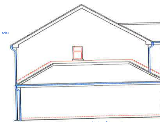
Proposed Side Elevation 1:100
