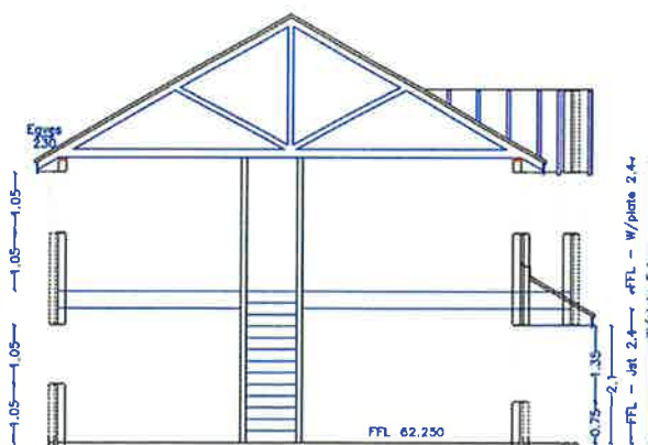
Proposed Section 1:150
