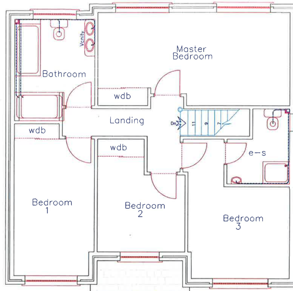
Proposed First Floor Plan 1:75
