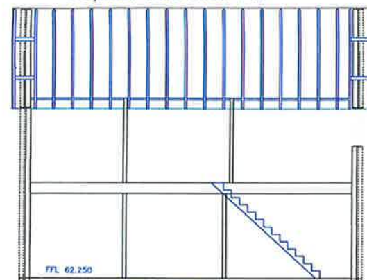
Proposed Section 1:150
