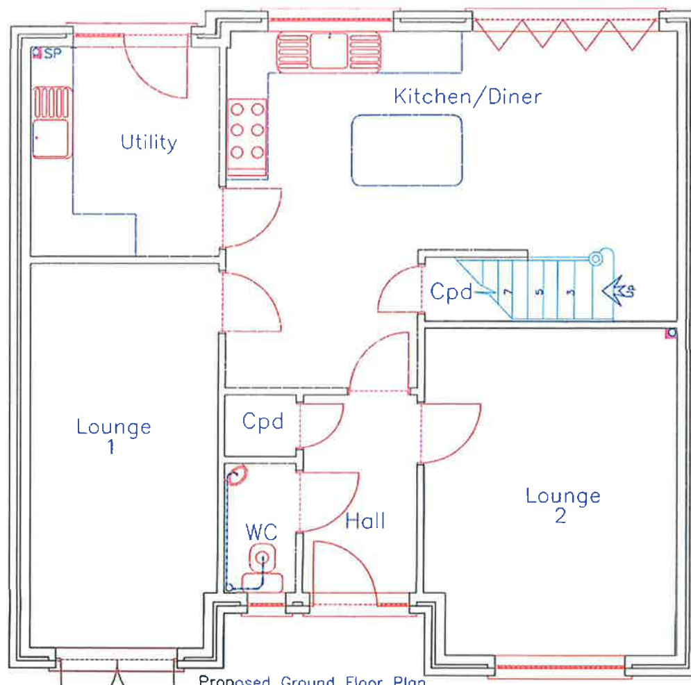
Proposed Ground Floor Plan 1:75
