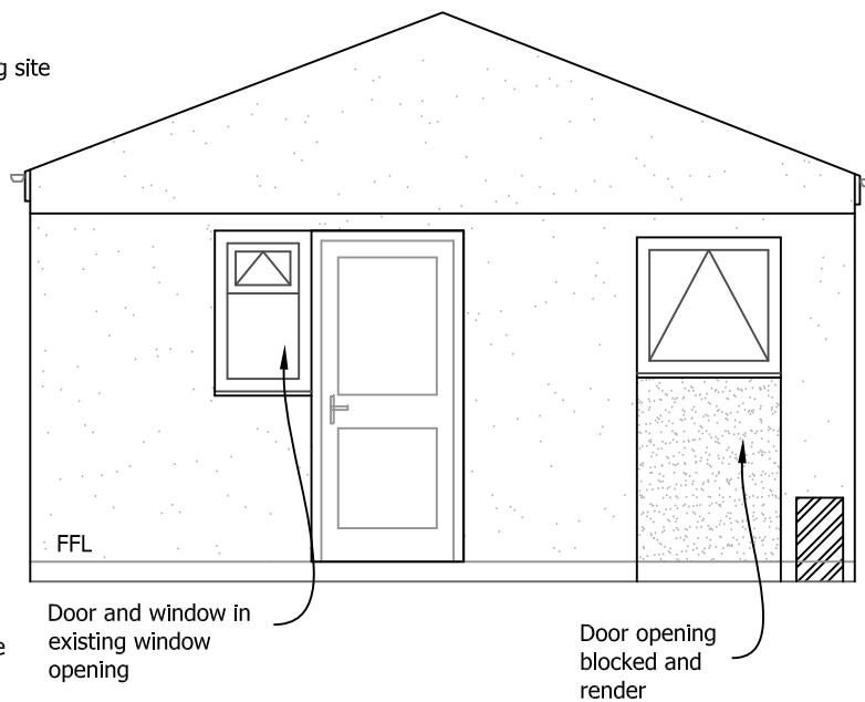
Right Elevation (House facing)
