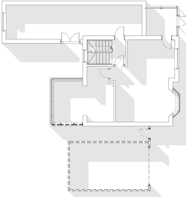
00 GF Demolition
