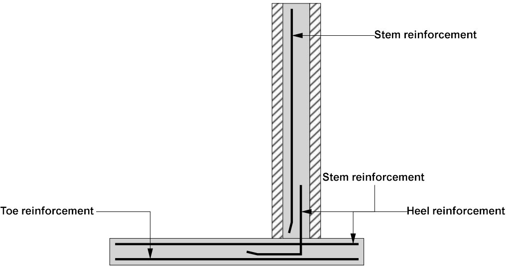
Indicative retaining wall reinforcement diagram
