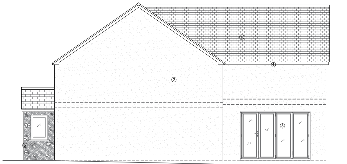
SIDE ELEVATION
