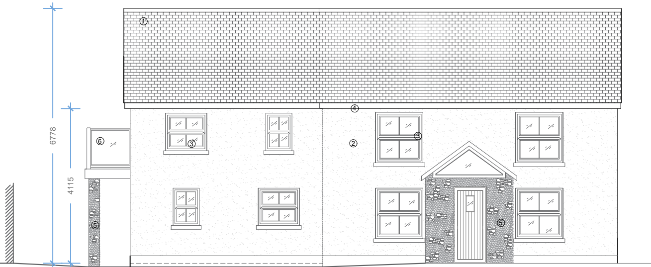
FRONT ELEVATION
