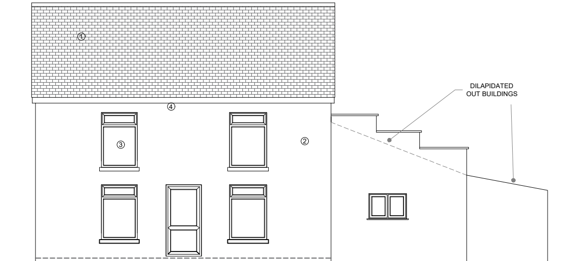
REAR ELEVATION
