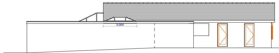
SIDE ELEVATION
