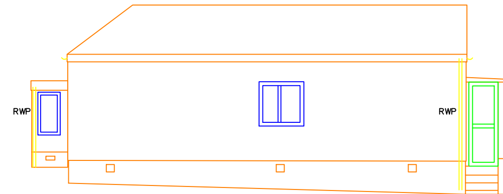
EXISTING SIDE ELEVATION (No Change)
