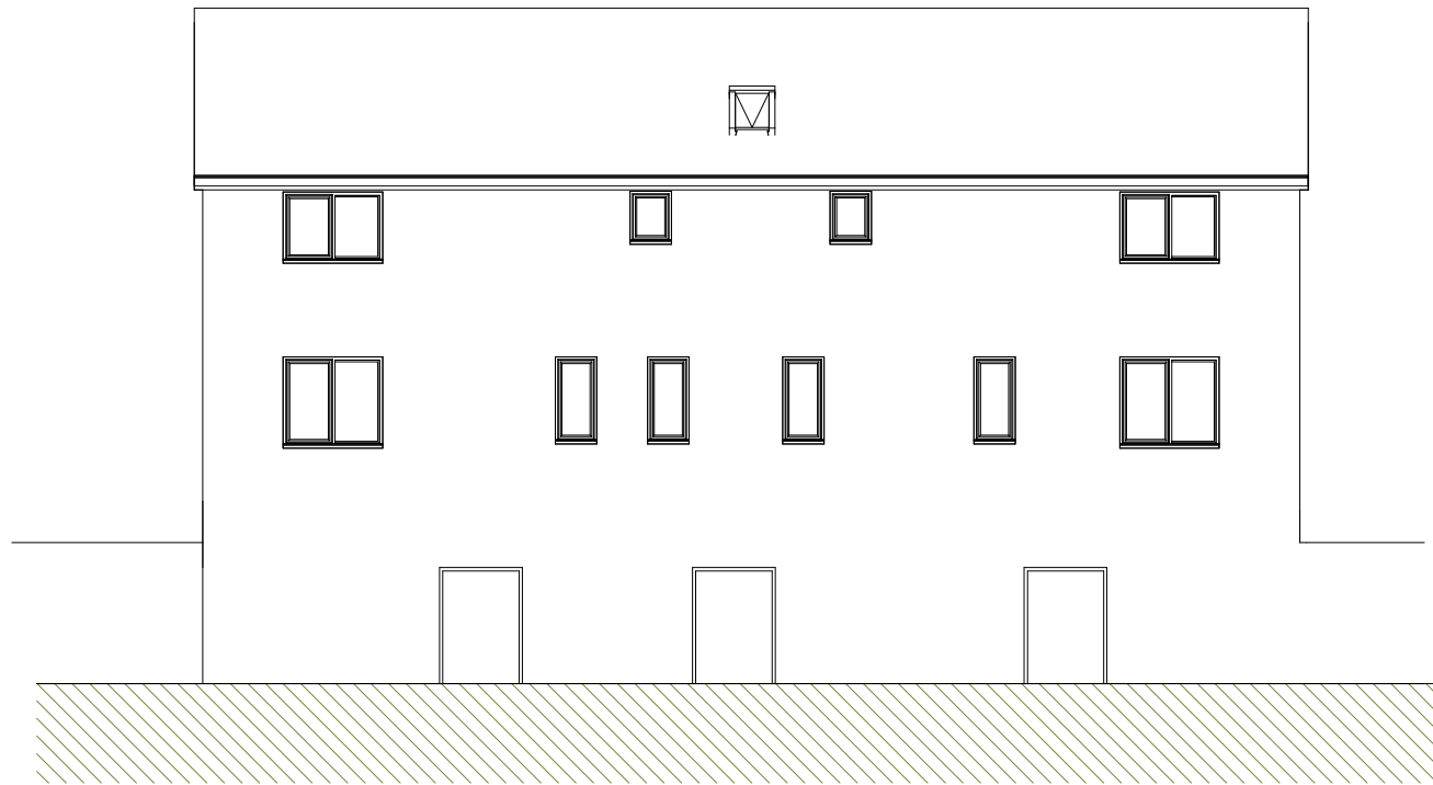
3 South West 1 : 100
