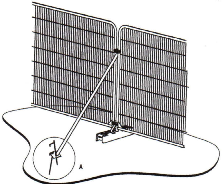
) Stabilizer strut with base plate secured with ground pins
