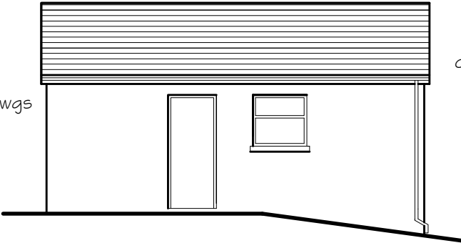
RH Side Elevation
