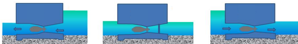
Figure 2.6: Illustration of water flow between the sea and the lagoon
