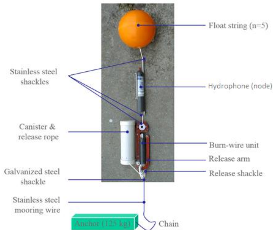
Figure 8.2 Fixed submerged listening station with automatic release mechanism
