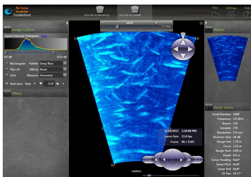
Figure 8.1 ARIS software
