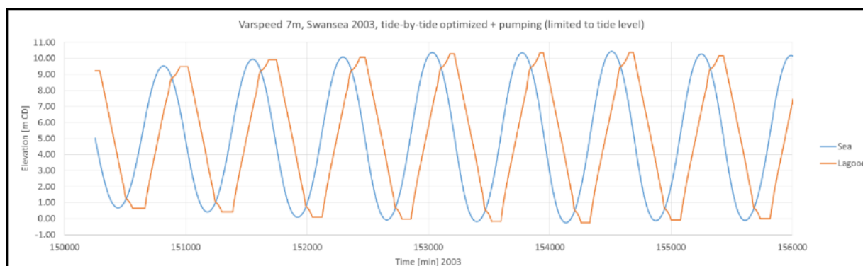
Figure 2.7: Indicative spring tide operating cycle for the lagoon
