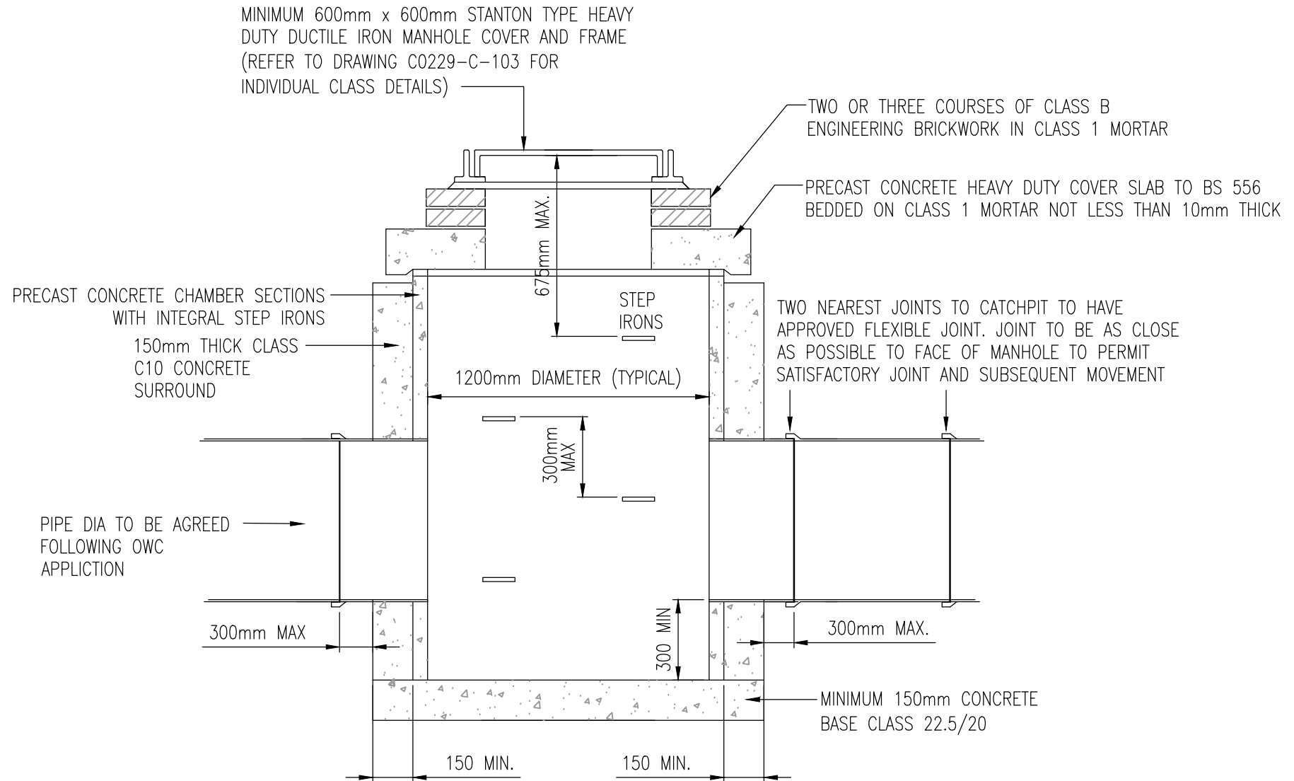
TYPICAL CATCHPIT MANHOLE SCALE 1:20
