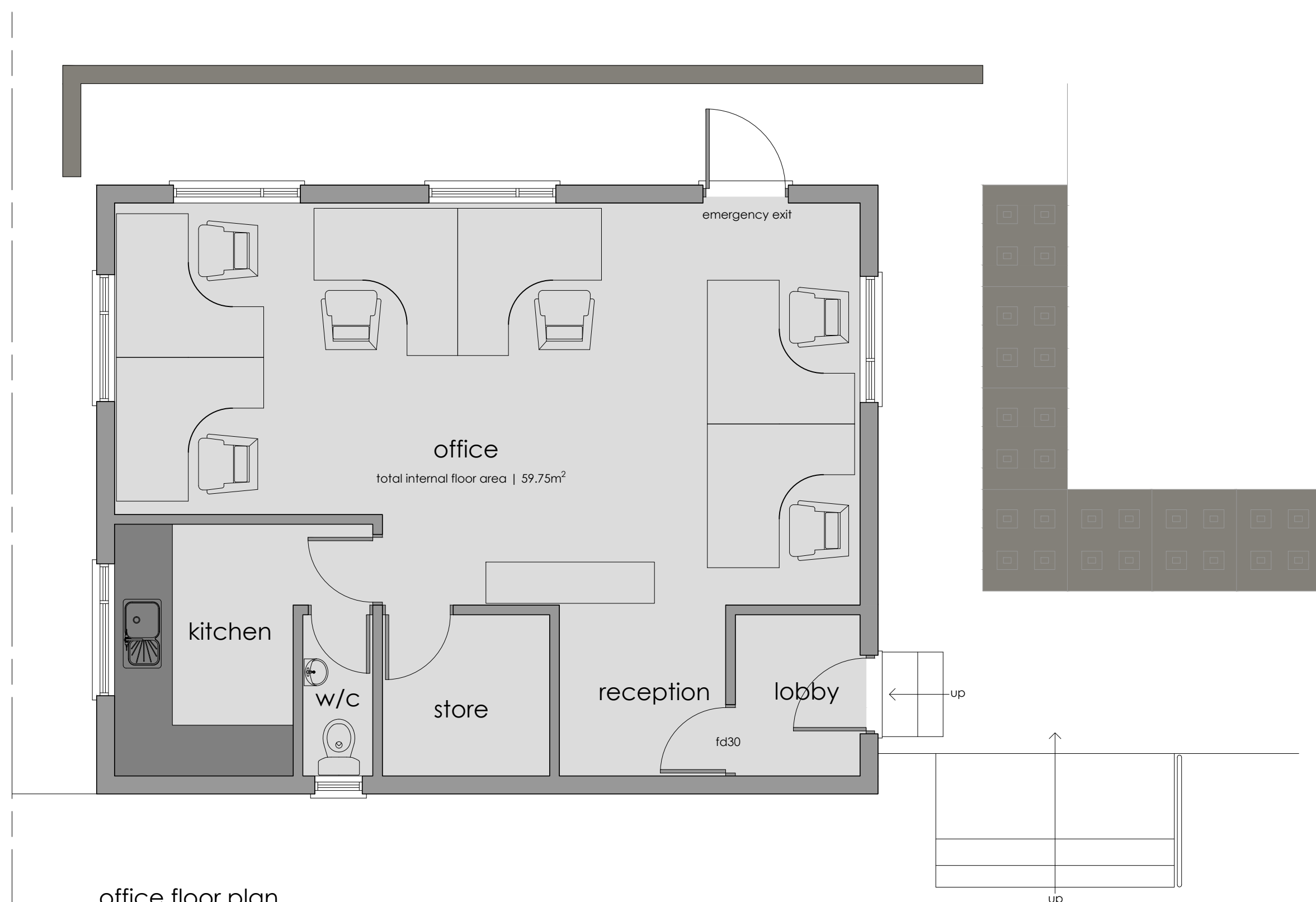
office floor plan scale | 1:50
